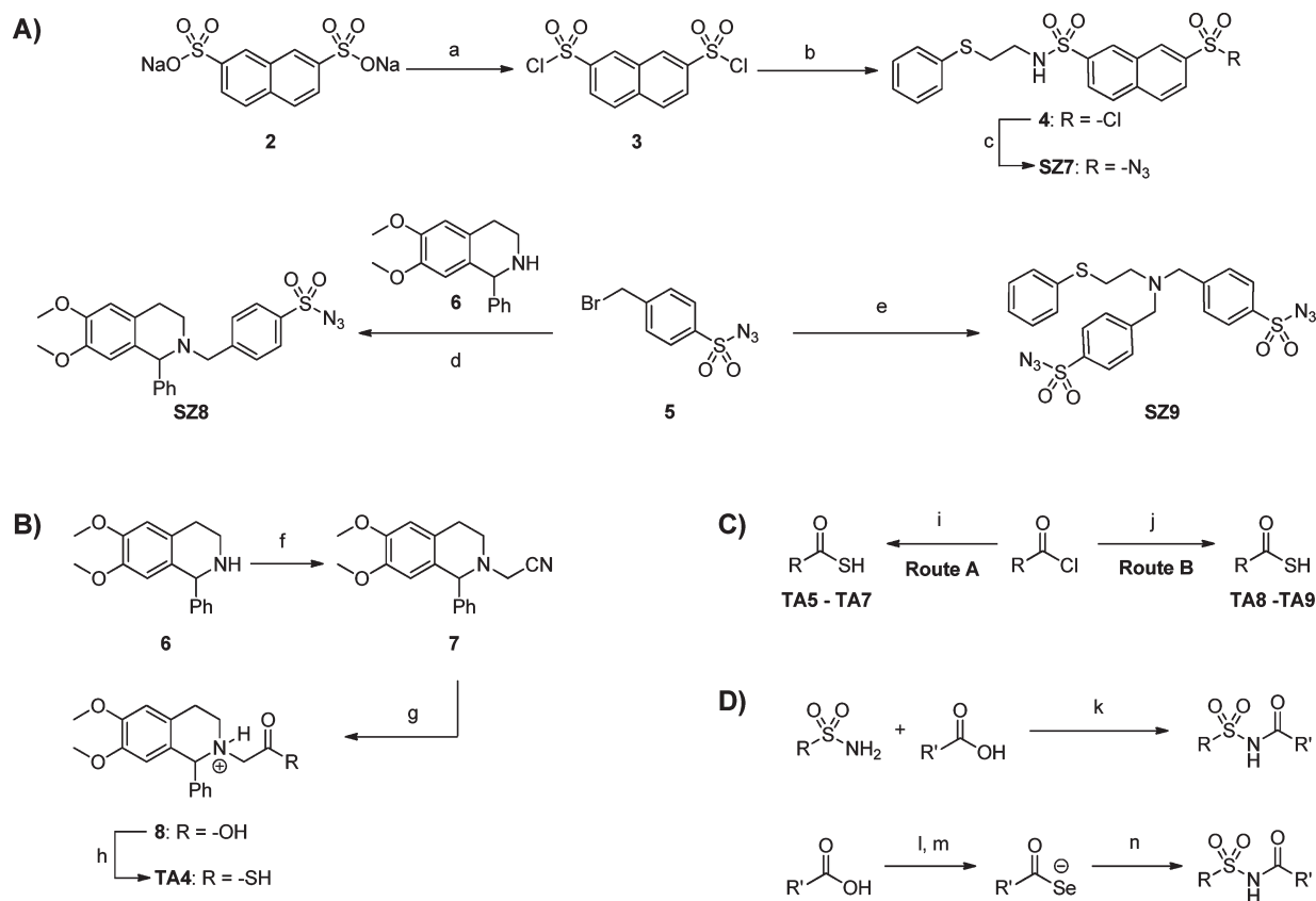
Figure 2. Synthesis of sulfonyl azides, thio acids, and acylsulfonamides. Reaction conditions: (a) SOCl 2 , DMF, reflux, 2 h; (b) 2-(phenylthio)ethanamine (0.5 equiv), K 2 CO 3 , CHCl 3 , 12 h, RT; (c) NaN 3 , acetone, H 2 O, 0 °C, 3 h, 70% (over 3 steps); (d) K 2 CO 3 , CH 3 CN/H 2 O (9:1), 12 h, RT, 87%; (e) 2-(phenylthio)ethanamine (0.5 equiv), K 2 CO 3 , CH 3 CN/H 2 O (9:1), 12 h, RT, 60%; (f) ICH 2 CN, K 2 CO 3 , CH 3 CN/H 2 O (10:1), 2 d, 60 °C, 79%; (g) 12 N HCl, 90 °C, 3 h, 66%; (h) (1) (COCl) 2 , CH 2 Cl 2 , 0 °C to RT, 8 h, (2) dimethylthioformamide, H 2 S, 15 min, 25%; (i) NaSH, acetone, H 2 O, 2 h, RT; (j) NaSH, neat, 0 °C to RT, 1 h; (k) EDCI, DMAP, CH 2 Cl 2 , RT, 24–48 h; (l) (CH 3 ) 2 CHOCOCI, N -methyl piperidine, THF, 0 °C, 30 min; (m) LiAlHSeH, THF, 0 °C, 30 min; (n) RSO 2 N 3 , THF, 0 °C to RT, 3 h.
