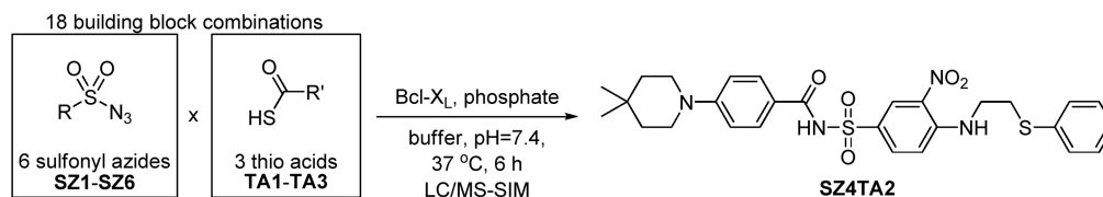
Figure 1. Kinetic TGS approach targeting PPIs. (A) TGS approaches are based on the principle that multidentate interactions between a ligand and a biological target are collectively much stronger than the corresponding monovalent interactions of each of the fragments. 60 Thus, a target-assembled compound most likely will have a stronger interaction with the biological target as compared to the individual building blocks. 60 In kinetic TGS, fragments decorated with complementary reactive groups are incubated with the target biomolecule. If two fragments reside simultaneously in close proximity in binding pockets of the target, the two reactive functionalities react with each other, forming a covalent linkage between the two fragments. (B) Acylsulfonamide 1, ABT-737, and ABT-263 compounds targeting Bcl-X L . (C) Proof-of-concept study to demonstrate that the amidation between thio acids and sulfonyl azides is suited for kinetic TGS targeting PPIs.
